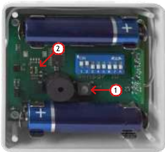
Fig. 4.3.5: Check functionality
