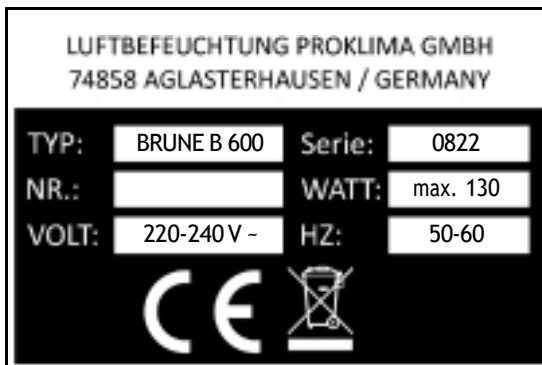
Fig. 11.6.1: Type plate
